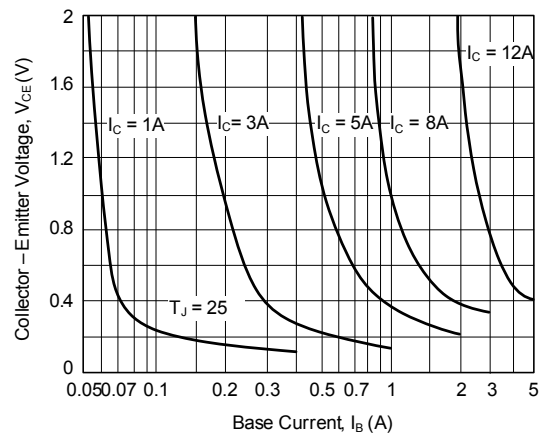
Figure 6. Collector Saturation Region
